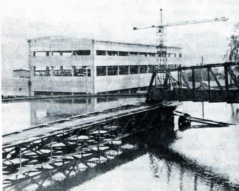
Titanium ore dressing plant under construction at the Panzhihua Iron and Steel Company, Sichuan Province.
